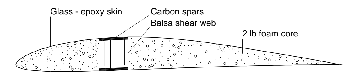
TYPICAL PROP SECTION: EPPLER 193
