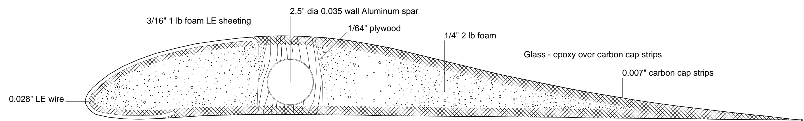
TYPICAL WING SECTION: MODIFIED LISSAMAN 7769
